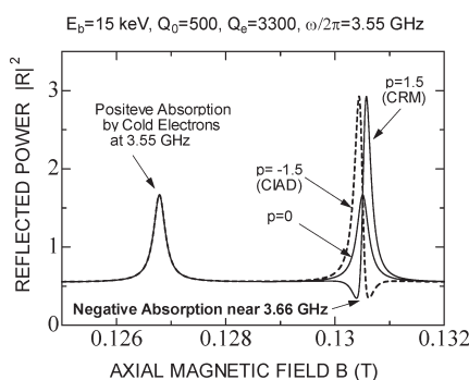
Fig. 2 Designed distribution of axial magnetic field of plasma-loaded CRM in TPD-II machine.
