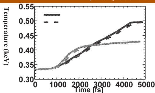
Fig. 1. Time dependent relativistic electron heat flux and heated core temperature
