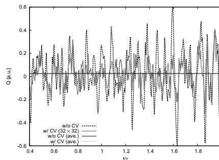
Fig. 2: Time evolution of the energy flux.
