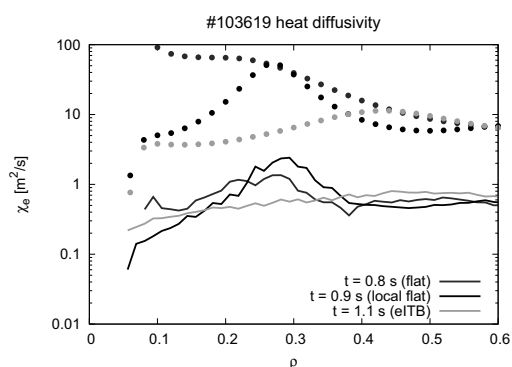
Fig. 1: Radial profiles of the thermal diffusivities in a CERC plasma at t = 0.8, 0.9, 1.1 s. Lines represent the neoclassical ones, and circles are the experimental ones.
