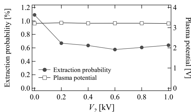
Fig. 2 Dependence of H - extraction probability and plasma potential on the lens voltage V_2
