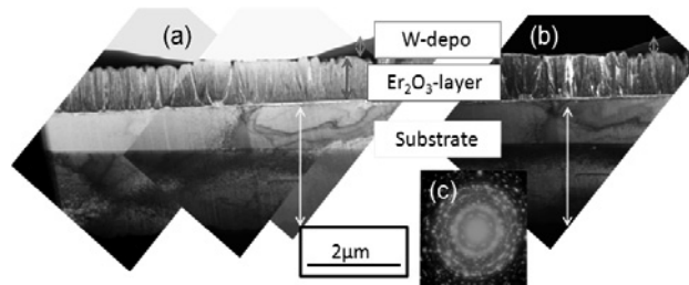
Fig. 2 TEM images obtained for the \text{Er}_2\text{O}_3 thin film on SUS316 steel before hydrogen permeable test. (a) a bright and (b) a dark field images.
