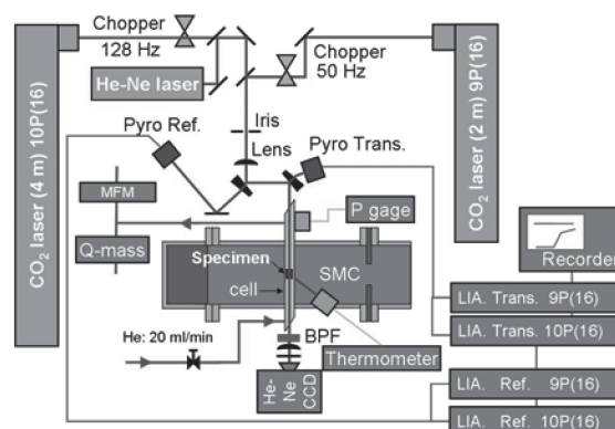
Fig. 1. Experimental setup of the microwave heating in the single mode cavity (SMC) and the LAS diagnostics system.
