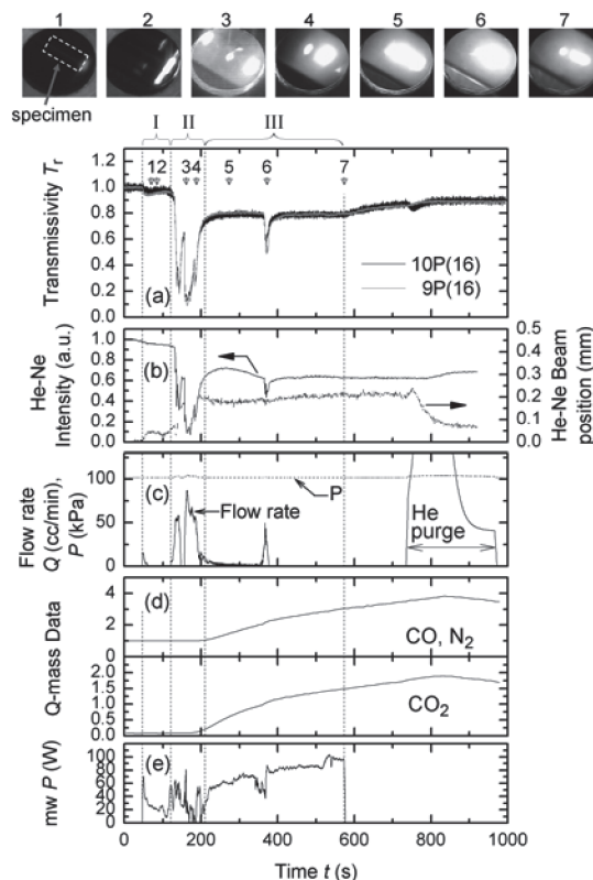
Fig. 2. Various time evolutions measured during the microwave carbothermic reduction of magnetite. CO 2 laser transmissivities in (a). Intensity of the transmitted He-Ne laser and its beam position in (b). Flow rate of exhaust gas and gas pressure in (c). Component intensity in CO and CO 2 measured by Q-mass in (d). Net absorbed power into the cavity in (e).
