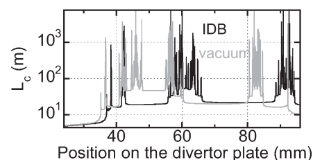
Fig. 2. Profiles of the connection length of the magnetic field lines on the divertor plate for vacuum (gray) and IDB (black) conditions, respectively.
