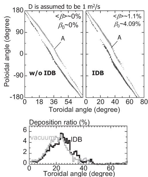
Fig. 3. (top) Simulated particle deposition profiles calculated by using field line tracing with the effect of diffusion. Poloidal angles of 0 and \pm 180 are outboard and inboard, respectively. (bottom) Toroidal angle distribution of particle deposition for the divertor trace “A” in top figures.
