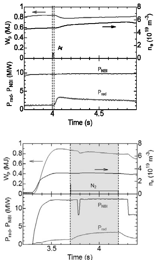
Fig. 1. Time evolutions of stored energy ( W_p ), line averaged density ( n_e ), NBI power ( P_{\text{NBI}} ) and total radiation power ( P_{\text{rad}} ) in typical Ar (top) and N 2 (bottom) seeded discharges, respectively.
