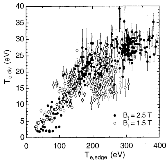
Fig. 3. T_{e,div} as a function of T_{e,edge}(\rho=1)
