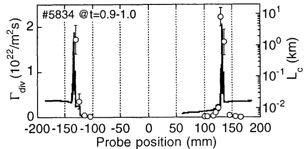
Fig.2 A profile of the particle flux to the divertor plate( \Gamma_{div} ) and connection length of magnetic field lines on which Langmuir probe and thermo-couple arrays are set. (#5834: Hydrogen discharge, NBI co and ctr. injection)
