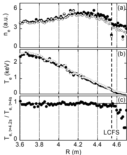
Fig. 2. Radial profiles of (a) electron density ( n_e ), (b) T_e before ( t = 4 s, \bullet ) and after ( t = 4.2 s, \circ ) Ne seeding, respectively, and (c) T_e ratio between after and before Ne seeding in the same discharge as Fig. 1.
