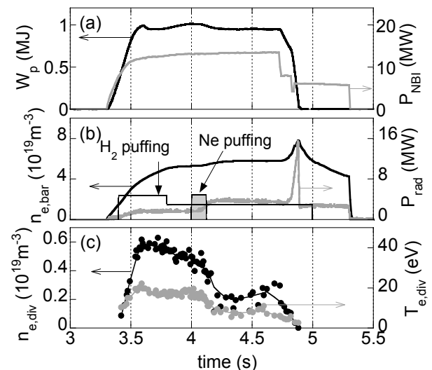
Fig. 1. Typical time evolutions of (a) plasma stored energy ( W_p ) and NBI power ( P_{NBI} ), (b) line averaged density ( n_{e,bar} ), radiation power ( P_{rad} ) and gas-puffing, (c) electron density ( n_{e,div} ) and temperature ( T_{e,div} ) in the divertor (torus inboard-side). (#103833, R_{ax}=3.60\text{m} , B_t=-2.8\text{T} , \gamma=1.2538 , B_q=100\% )
