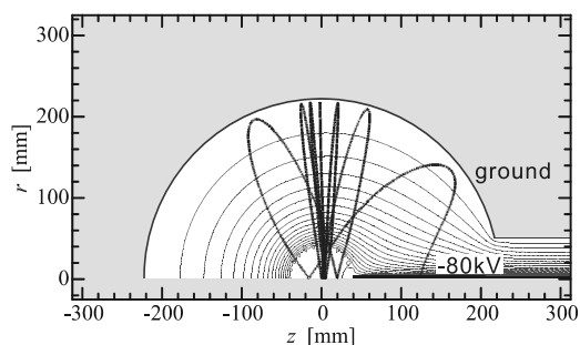
Fig. 3. Calculated potential contours and an ion trajectory. The ion is seen to hit the high-voltage feedthrough rod after five oscillatory motions.
