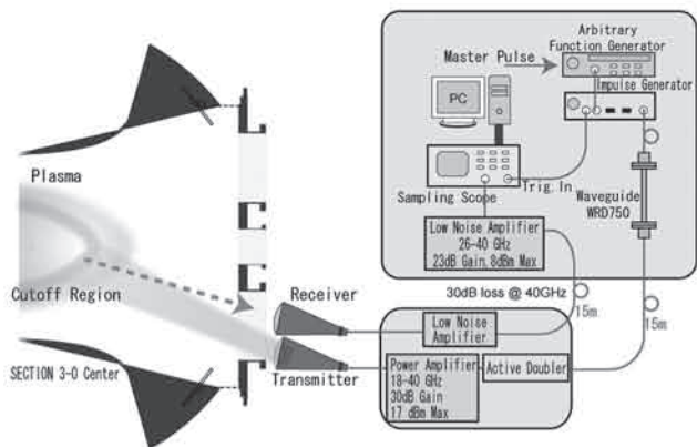
Fig. 1 Schematic of the USRM system.
