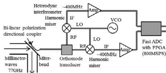
Fig. 1. Schematic of power/polarization monitor for EC waves.
