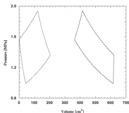
Fig. 2 P - V diagram of the pulse-tube
