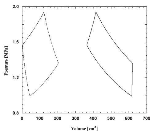
Fig. 2 P - V diagram of the pulse-tube
