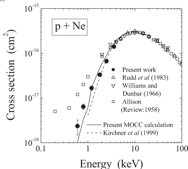
Fig. 1. Charge-transfer cross sections for H^+ ions in collisions with Ne atoms.
