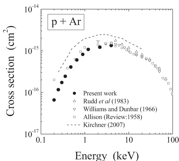
Fig. 2. Charge-transfer cross sections for H^+ ions in collisions with Ar atoms.
