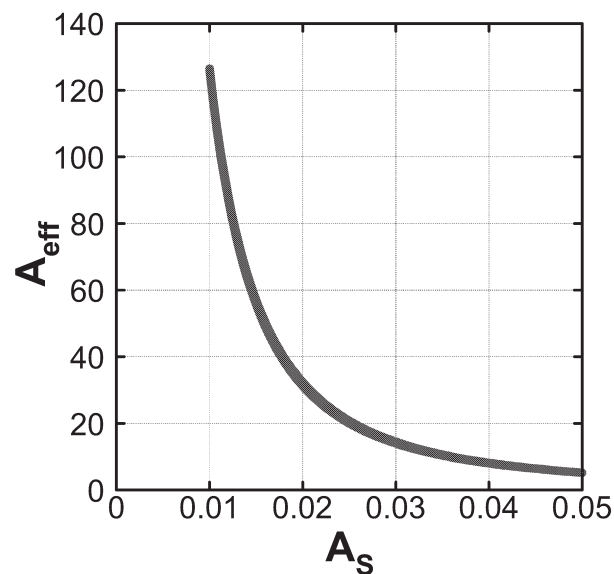
Fig.3 Dependence of A_{eff} on normalized length of short stub tuner.
