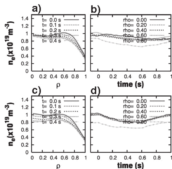
Fig. 1. Density profile at several time slices after ECH injection [ a) and c) ]. Time evolutions of the density at several spatial points b), and d) for ripple top [ a) and b) ] and bottom [ c) and d) ] heating cases.
