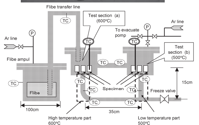
Fig. 1 Flibe loop and ampul
