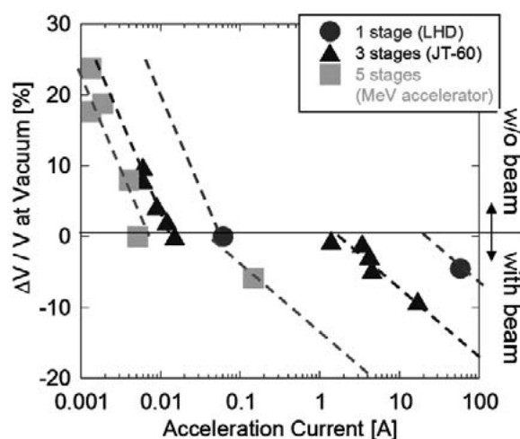
Figure 2. Voltage degradation characteristics depending on acceleration current. V denotes the acceleration voltage.
