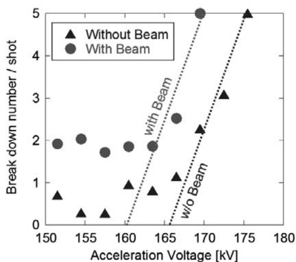
Figure 1. The breakdown probability of LHD-NBI3
