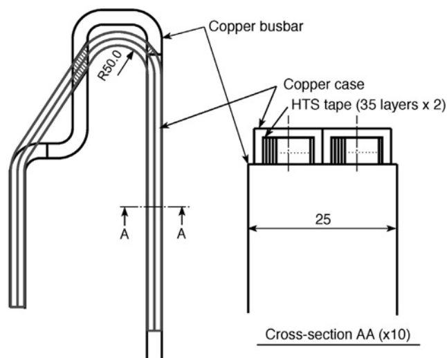
Fig. 2. Additional busbars with HTS tape conductors on the side of the copper busbar.
