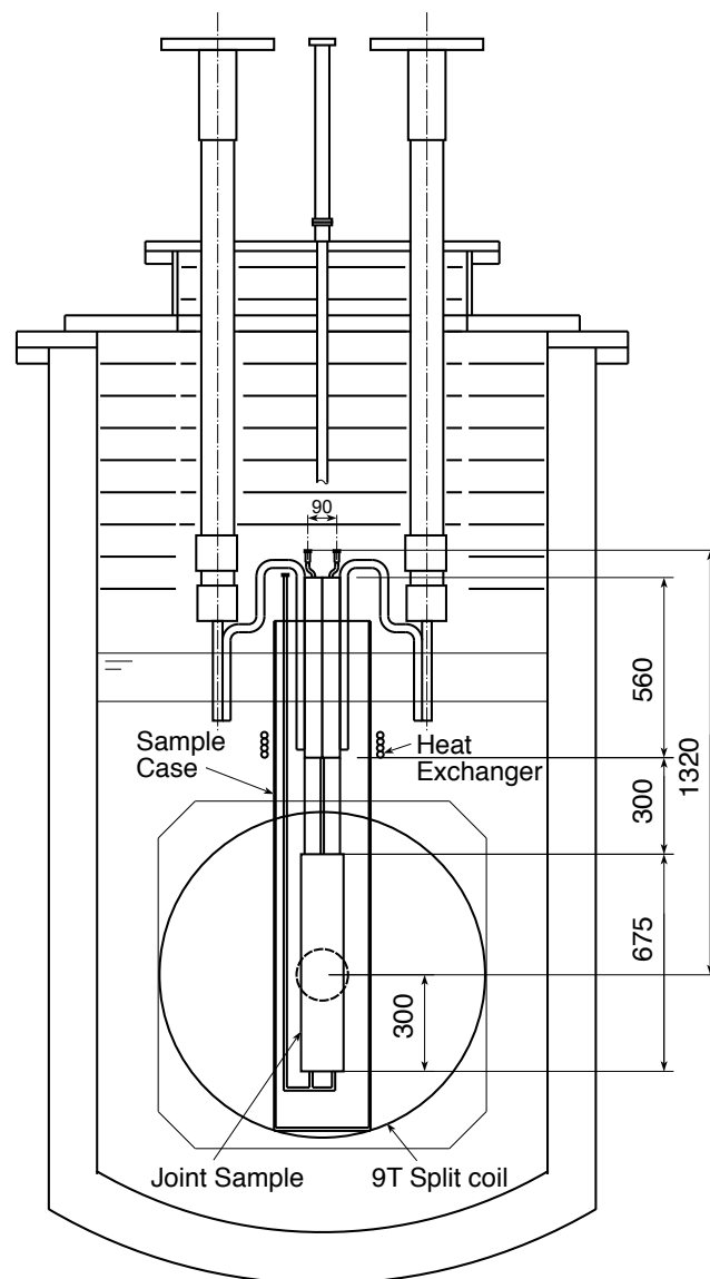
Fig. 1. Set up of an ITER-TF joint sample in the conductor test facility with 9 T split coils.
