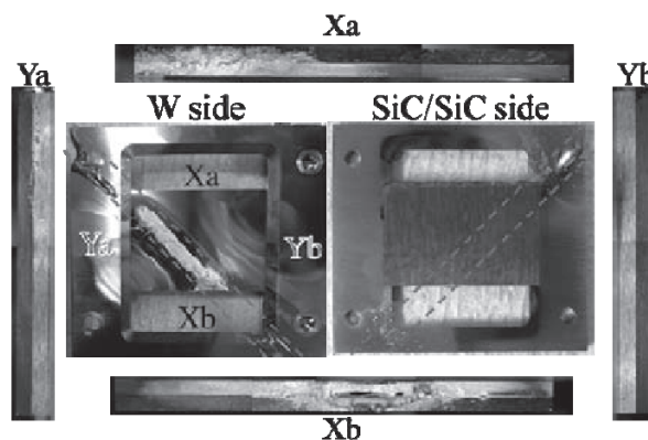
Figure 2. Surface Morphology after Plasma Exposure
