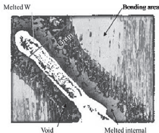
Figure 3. The Result of Ultrasonic Test
