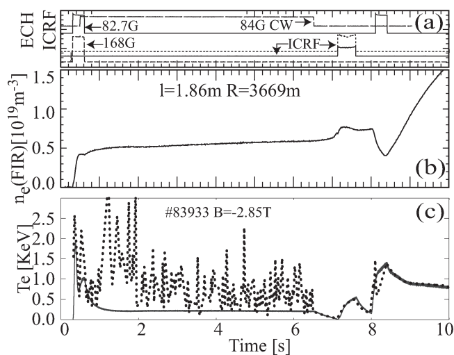
Fig. 2 Time sequence of the heating systems (a), electron density measured by the FIR interferometer(b), and time traces of electron temperature (c) measured by the radiometer (solid line) and Michelson spectrometer (dotted line).
