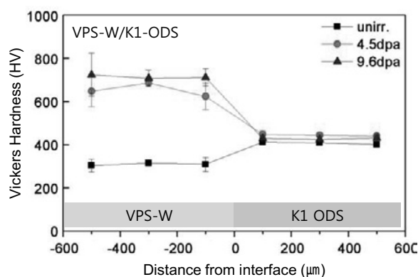
Fig. 2: The effect of neutron irradiation on the hardness of W-plasma sprayed ODS steel.
