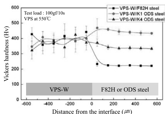
Fig. 1: The hardness distribution across the joint boundary of VPS-W and substrate materials.
