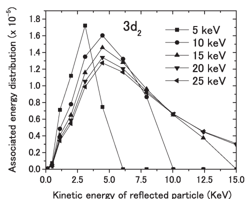
Fig. 1: Associated energy distribution of 3d_2 state in neutral D atoms reflected at Mo surface with an emission angle of 60 degree to the surface normal. The distributions are shown for five incident energies in 5-25 keV and an incident angle of the 60 degree.
