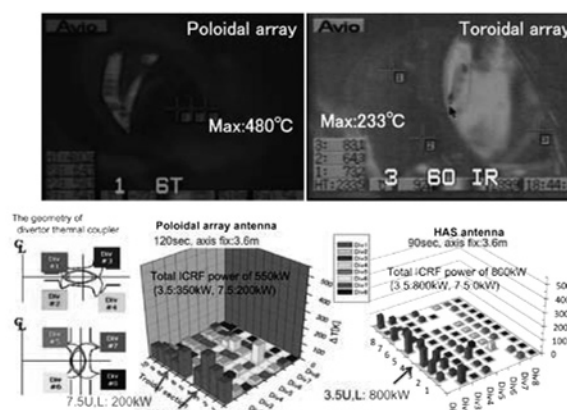
Fig. 2. The comparison with local hot spots on the antenna protectors (Infrared camera) and the increments in thermocouple on divertor tiles between poloidal array antenna and toroidal array antenna. Antenna plasma distances between last closed flux surface and antenna protectors are 12 cm for poloidal array antenna and 7 cm for toroidal array antenna.
