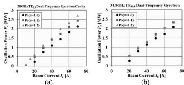
Fig.2 Beam current dependences of cavity oscillation power of dual-frequency gyrotron with each electron beam pitch factor \alpha (a) 28 GHz TE_{8,5} mode (b) 34.8 GHz TE_{10,8} mode.
