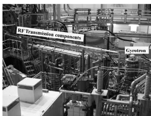
Fig.1 Picture of the gyrotron and transmission wave guide installed at QUEST
