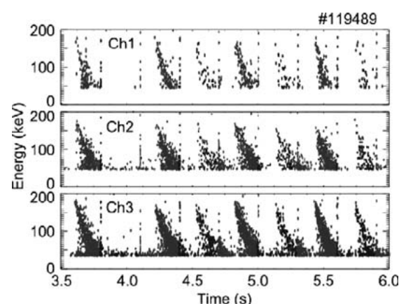
Fig. 3. The time evolution of the observed particle energy. The local energy decay process was observed.
