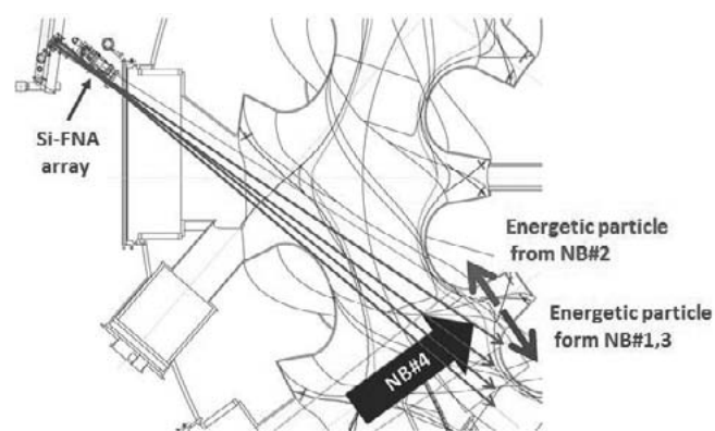
Fig. 1. Schematic view of the developed Si-FNA high energy particle measurement system.
