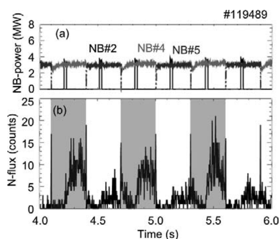
Fig. 2. Time evolution of the (a) NB-power and (b) N-flux. (a) Two NBs #4 (red) and #5 (blue) were used alternately for plasma sustain. The short pulse NB#2 was injected in red and blue timing in order to supply high energy test particles, (b) the flux was observed.
