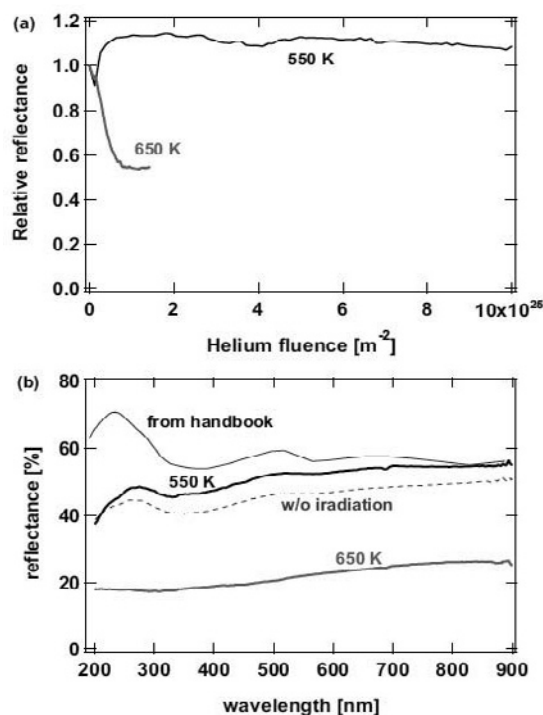
Fig. 1. (a) shows a temporal evolution of the relative optical reflectance at 633 nm at two different surface temperatures, i.e. 550 K and 650 K. (b) shows the wavelength dependence of the optical reflectance of Mo samples without and with the exposure to the plasma.
