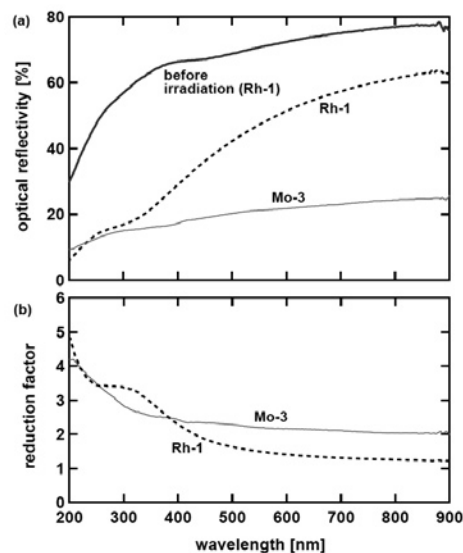
Fig. 2 (a) Wavelength dependences of the optical reflectivity of rhodium and molybdenum samples before irradiation and after helium irradiation (Rh-1 and Mo-3) are shown. (b) Wavelength dependence of the reduction rate of optical reflectivity for Rh-1 and Mo-3. The irradiation temperatures for Rh-1 and Mo-3 are 600 and 850 K, respectively.
