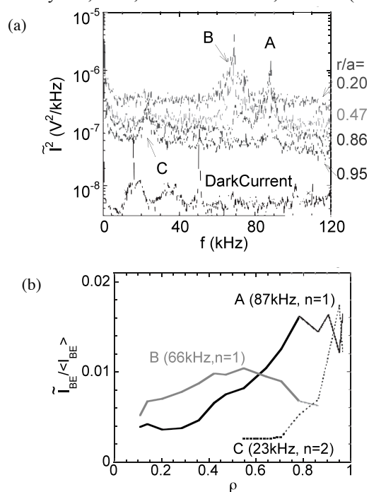
Fig. 2. (a) Power spectra of the beam emission at r/a=0.20-0.95 obtained in the NBI heated plasmas of Heliotron J (#46382, #46392), and (b) radial profile of the beam emission fluctuation for the mode A-C.
