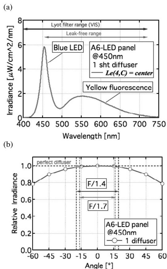
Fig. 1 Optical properties of flat white-color LED panes of A6 size. (a) Spectral irradiance (b) relative angular distribution of the irradiance at 450 nm. Note that the irradiance exhibits unity for perfect diffuse reflector, since radiance shows cosine while the observing area shows reciprocal of the cosine dependence on the observing angle.
