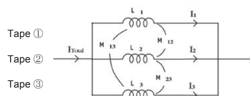
Fig. 5 Simple equivalent circuit of a 3-strand parallel conductor.
