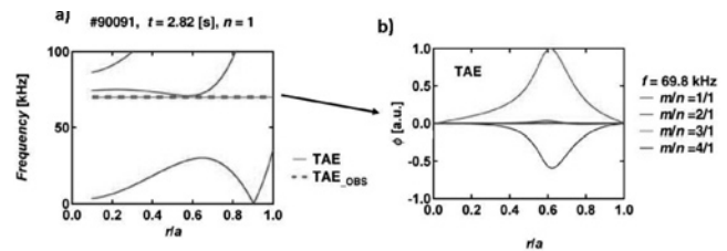
Fig. 2. a) Shear Alfvén spectra ( n=1 ) calculated by the STELLGAP code. b) Eigenfunction of the TAE mode calculated by the AE3D code.
