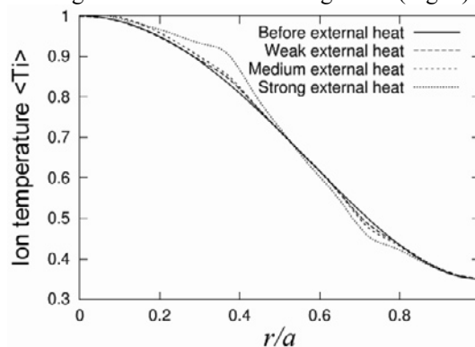
Fig. 1. Ion temperature profile averaged over poloidal and toroidal angles before the additional heating and after in case 1. The profile does not change around r/a=0.5 for the weak heating and the medium heating, while it changes for the strong heating.
