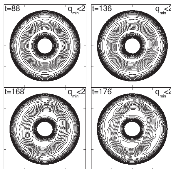
Fig.2. Time evolution of the equi-contour of helical flux of m/n=2 on the same poloidal section. The magnetic islands of macro-MHD appear appears at t=168 .
