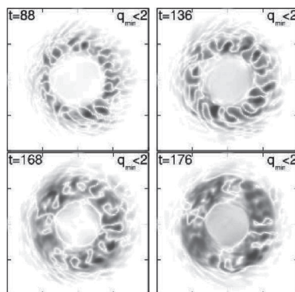
Fig.1. Time evolution of the electric potential on the same poloidal section. The first frame shows quasi-steady equilibrium. The macro-MHD appears at t=168 .
