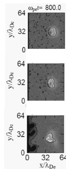
Fig. 2: Electron density distributions in the x - y plane at z = L_z/2 at \omega_{pe}t = 800 where the magnetic strength is set as |\Omega_e|/\omega_{pe} = 10, 5, and 1 in the upper, middle, and bottom panels, respectively.
