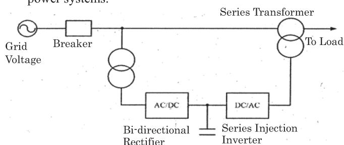
Fig.1. Configuration of the of High Quality B1 Supply System.
