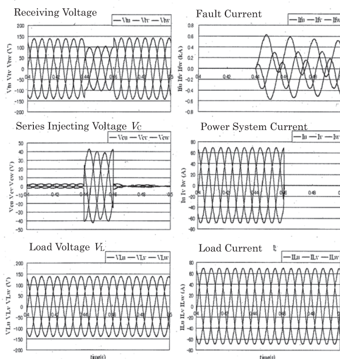
Fig.3. Simulation Result of High Quality B1 Supply System.
