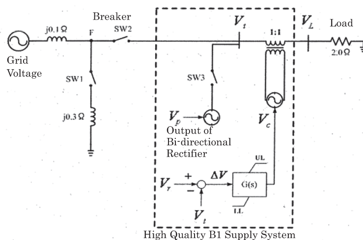
Fig.2. Simulation Model of High Quality B1 Supply System.
