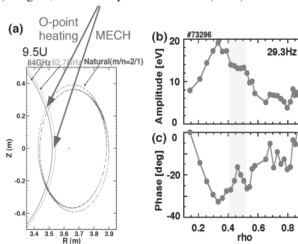
Fig. 1. (a) Typical configuration in experiments. Modulated EC wave was injected in the core region, and at the same time unmodulated EC wave was injected in the island region. (b) Amplitude profile and (c) phase profile at the modulation frequency.
