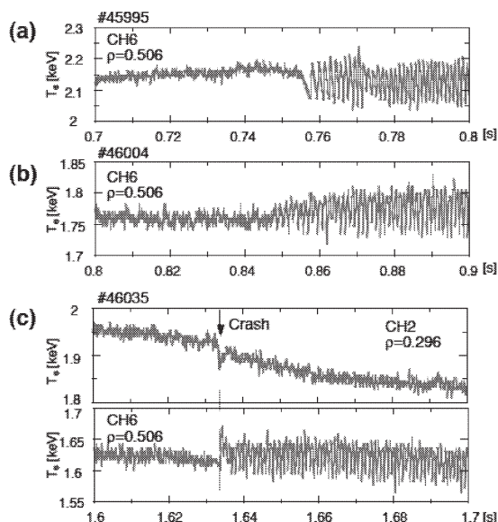
Fig. 2. Temporal evolution of electron temperature near \nu/2\pi \sim 0.5 at the onset of sinusoidal oscillations: (a) fast growth, (b) slow growth, (c) sawtooth-triggered oscillations.
