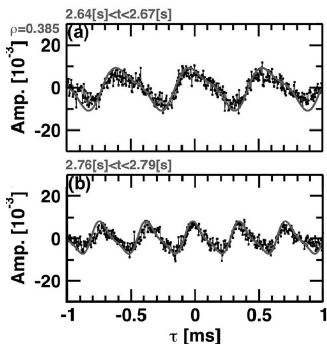
Fig. 2 Reconstructed periodic non-sinusoidal waveform (black curves) at two different time windows. Bi-spectrum-filtered signals are also shown (red bold curves).
