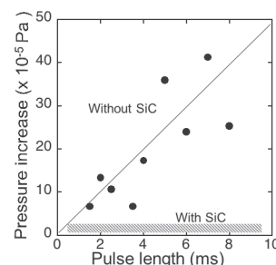
Fig. 1 Pressure increase during the high power transmission in MOU with and without SiC..
