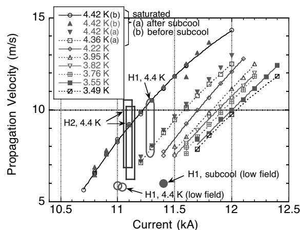
Fig.1. Comparison of propagation velocities in the LHD helical coil and the model coil.
