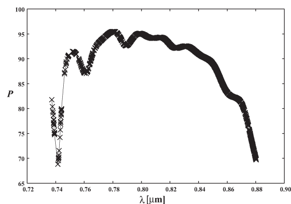
Figure 2: The values confined ratio of light as a function of wave length of light. R = 0.4148663\mu\text{m} , r = 0.1031004\mu\text{m} .
