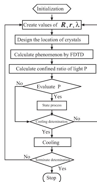
Figure 1: The algorithm for calculating optimal parameters for the design of the photonic crystal with photonic band gap.
