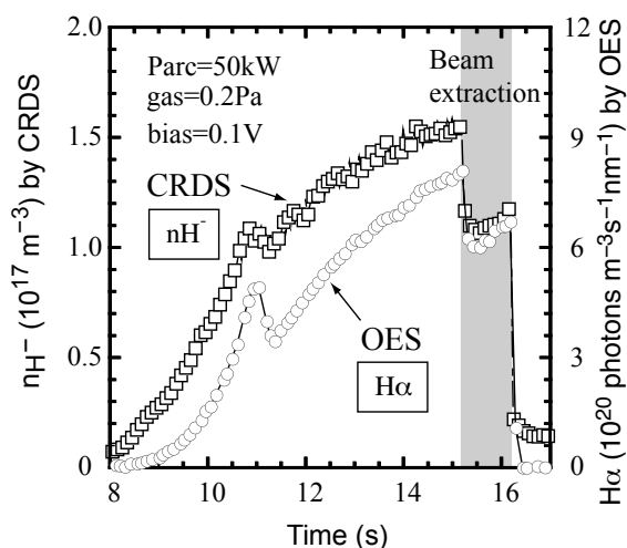
Fig. 1: Time evolution of H^- density measured by CRDS (squares) and H_\alpha emission intensity measured by OES (circles) in arc discharge. Both of which dropped during beam extraction (gray area).
