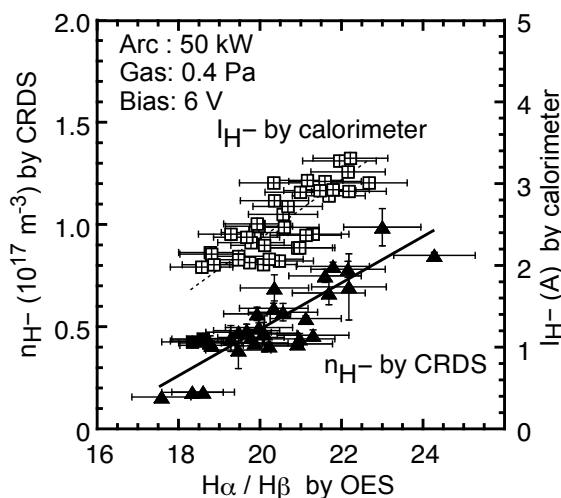
Fig. 2: Correlations of H_\alpha/H_\beta measured by OES with H^- ion density measured by CRDS in the extraction region and with the H^- beam current measured by the beam calorimeter. The condition of arc discharge is constant with different Cs conditions.
