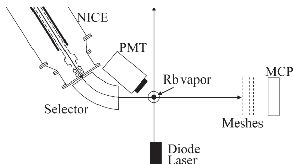
Figure 1: The experimental apparatus
