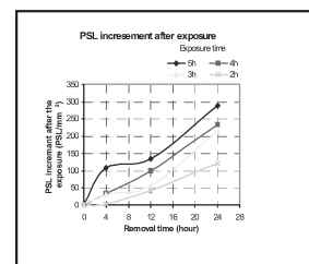
Fig.4 PSL increment after exposure with removal time
