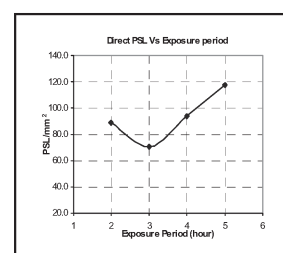
Fig.6 Relationship between photon dose and PSL value increment after exposure
