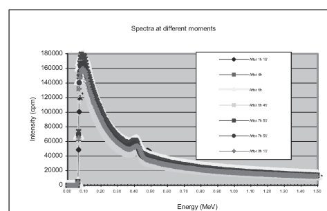
Fig.7 Photon spectra at reference point of reactor
