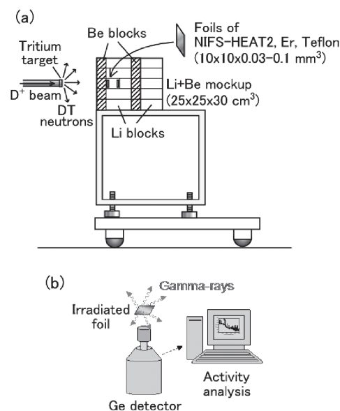
Fig. 1. Schematic drawings of (a) DT neutron irradiation with Li+Be mockup for radioactivity evaluation of blanket materials and (b) activity analysis with Ge detector.
