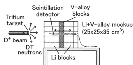
Fig. 2. Schematic drawing of DT neutron irradiation with Li+V-alloy mockup planned for evaluation of neutron transport and tritium production in Li/V-alloy blanket system.
