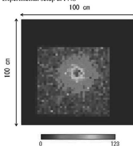
Fig.2 Reconstructed image of DT neutron at the source position
