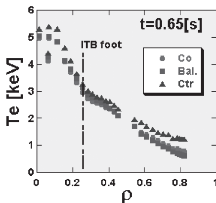
Fig. 3: Electron temperature profiles in the co-, balanced and counter injections.
